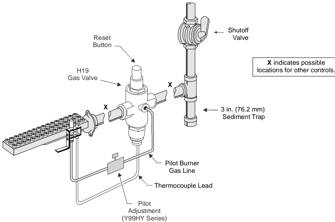
Figure 1: Typical H19 Gas Valve Installation
